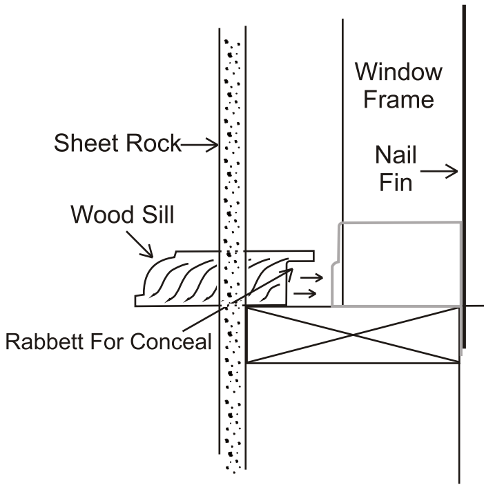
Window Detail For Wood Sill
