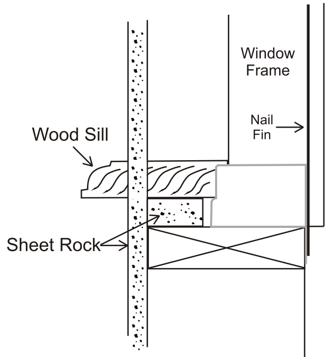
Window Detail With Wood Sill over Sheetrock Furring
