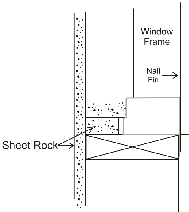
Window Detail For Sheet Rock Sill
