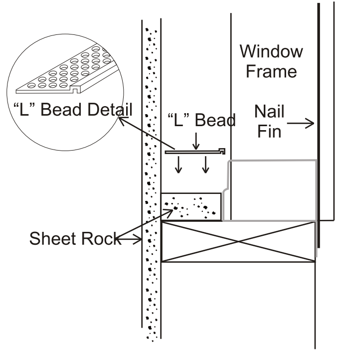
Window Detail For Sheet Rock Sill
